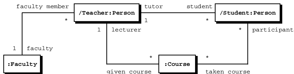
Figure 2: A typical UML collaboration with classifier roles shown as boxes (taken from [48]). The name after the slash is the name of the classifier role, and the name after the colon is that of the type (class) on which the role is based. Note that :Faculty and :Course provide no explicit role names. (See [67] for a complete discussion of roles in UML.)
