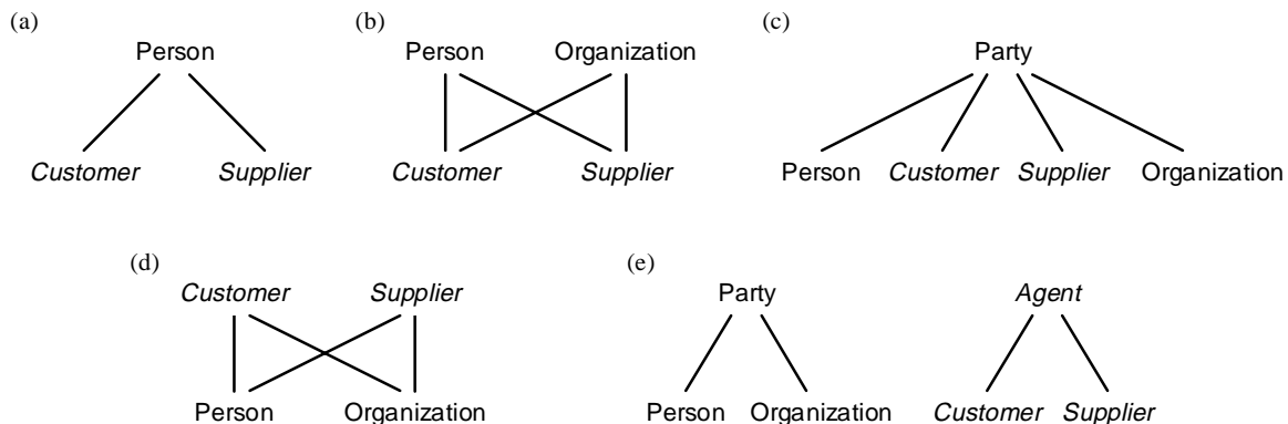
Figure 1: Relating roles and types through subtyping (roles are italicized).
