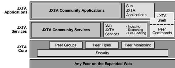
Figure 1. JXTA Layers
