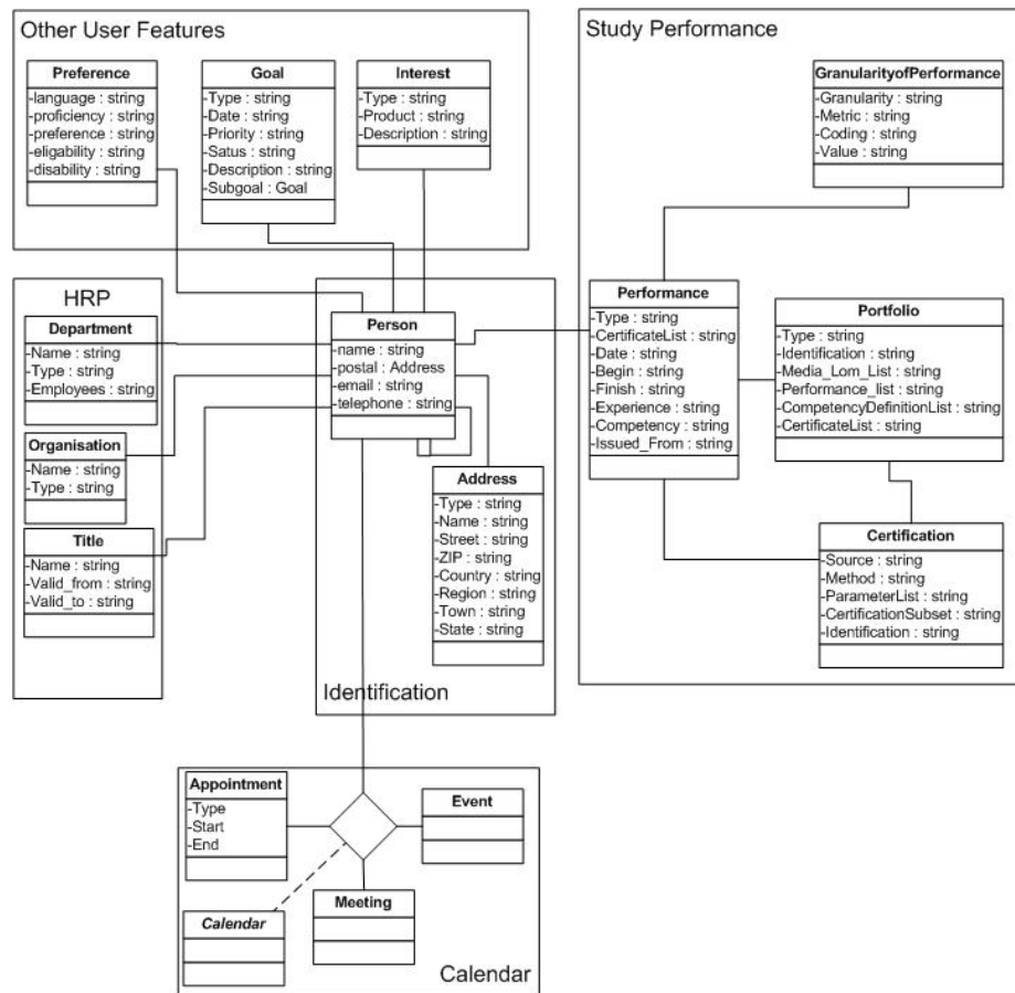
Fig. 3. First version of conceptual model of user profile for Elena.
