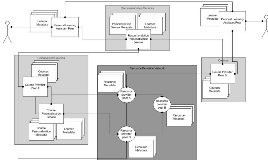
Fig. 4. ELENA architecture for personalization services.
