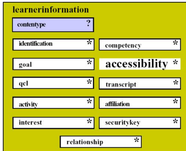
Fig. 2. The core categories for learner data in IMS LIP [5].
