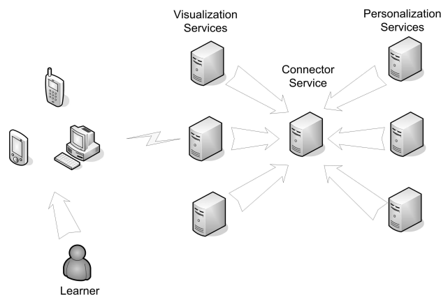
Figure 1: Architecture
